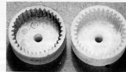
Left: A stone in the works destroys teeth! Keep the cover on. Right: The annular ring gear as new.
